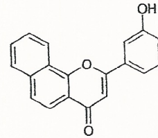
Chromatogram 3'-Hydroxy-alpha-naphthoflavone D:\promonence\Data\2013\APR-2013\030413S.lcd
