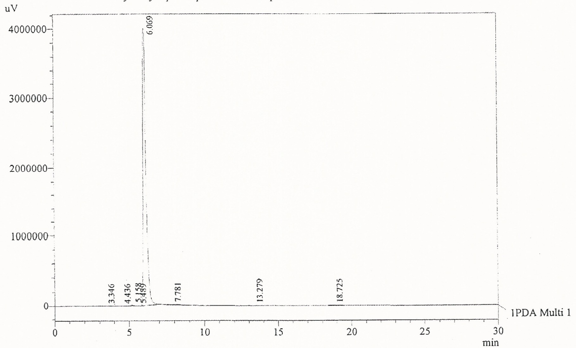
Chromatogram 3'-Hydroxy-alpha-naphthoflavone D:\promonence\Data\2013\APR-2013\030413S.lcd
